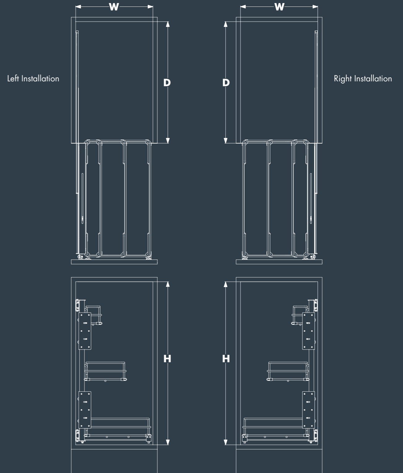
Inner Installation Dimensions
