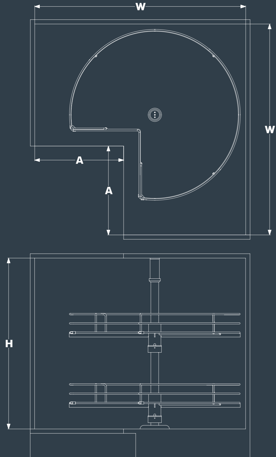
Inner Installation Dimensions
