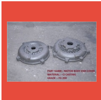
Casting Parts
